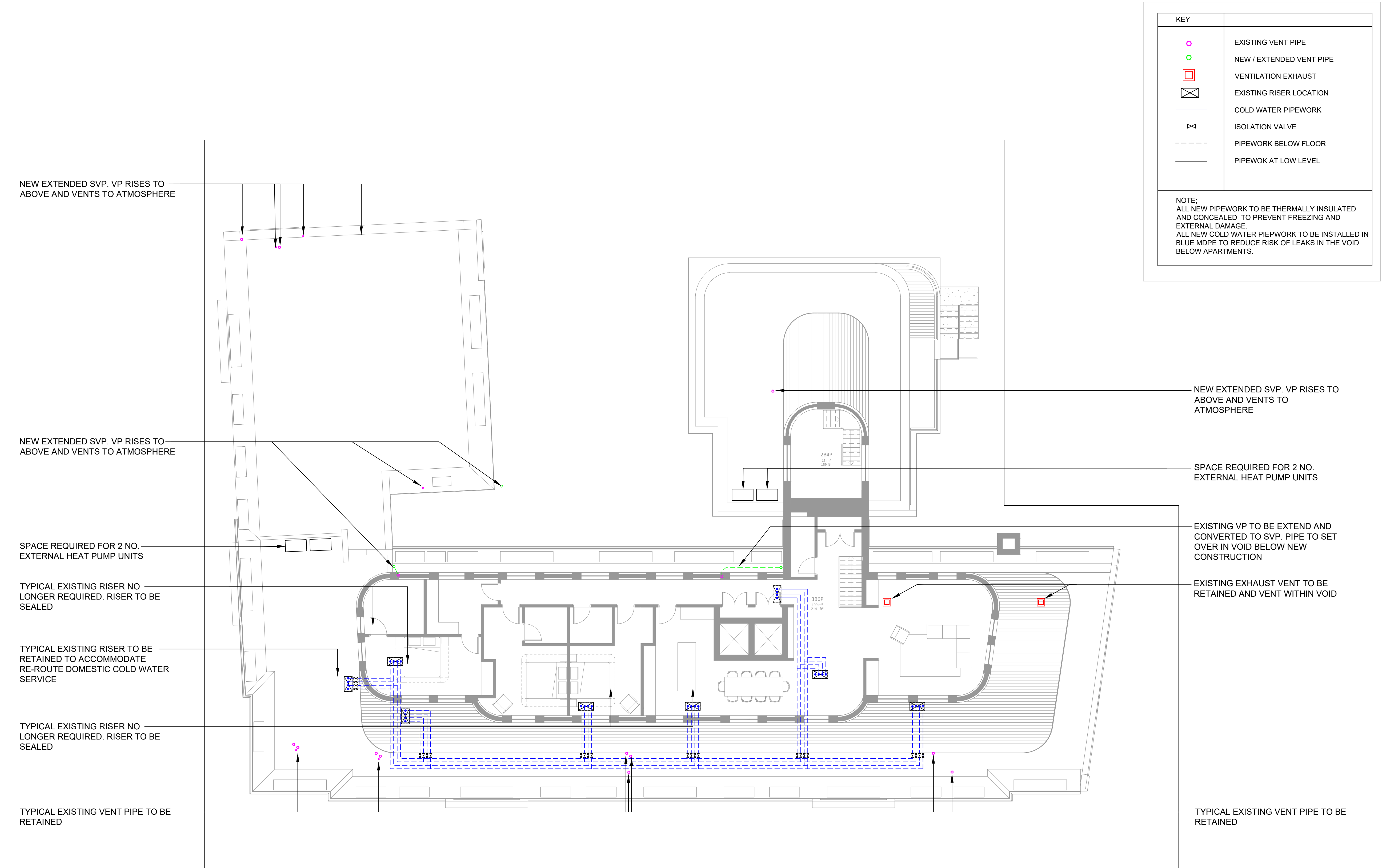
9TH FLOOR PLAN LAYOUT - PROPOSED
